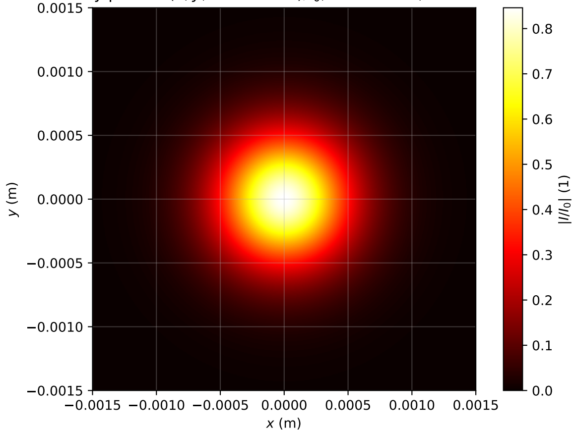
Intensity profile I(x, y, z = 1.592m)/I_0 , Pin=0.4Pcr, artificial time
